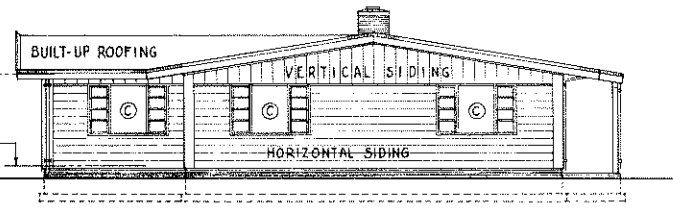
BED-ROOM-END-ELEVATION SCALE 0 4 8 12 FT.
