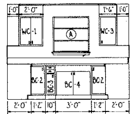
ELEVATION-B
