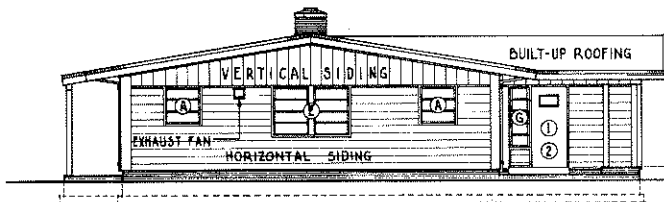
FAMILY-ROOM-END-ELEVATION SCALE 0 4 8 12 FT.
