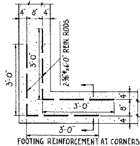
FOOTING REINFORCEMENT AT CORNERS
