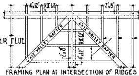
FRAMING PLAN AT INTERSECTION OF RIDGES
