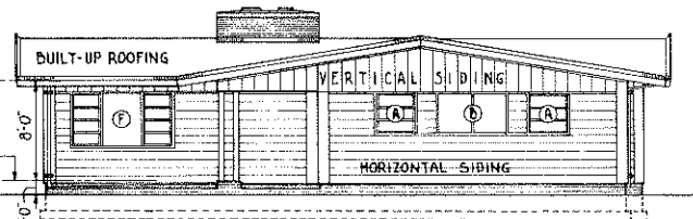
FRONT-ELEVATION SCALE 0 4 8 12 FT.
