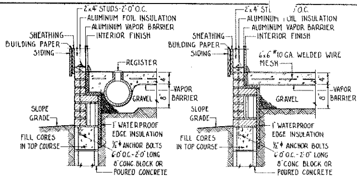
TYPICAL DETAIL OF PERIMETER HEATING LINE
