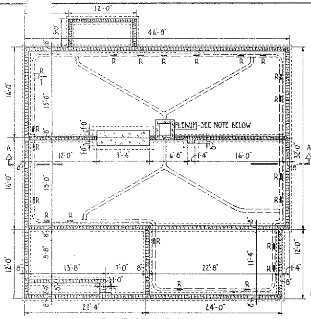
FOUNDATION PLAN
