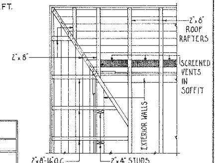
PLAN OF SOFFIT FRAMING SHOWING BOARD FINISH ON UNDER SIDE SCALE 0 1 2 3 FT.
