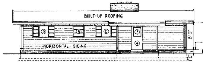
REAR-ELEVATION SCALE 0 4 8 12 FT.
