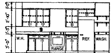
ELEVATION "A"
