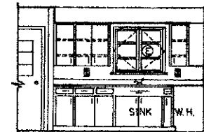
ELEVATION "B"
