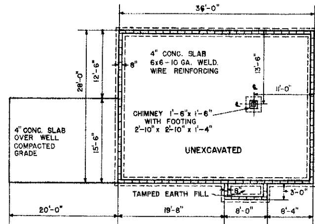
FOUNDATION PLAN SCALE 1/4" = 1'-0"
