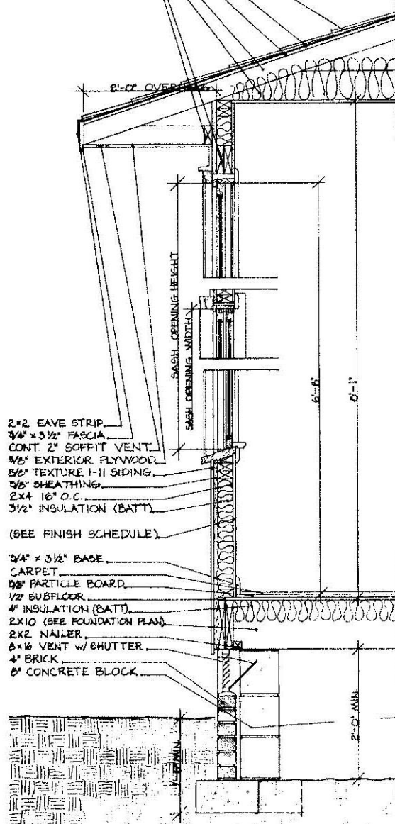
TYPICAL WALL SECTION SCALE: 1" = 1'-0"
