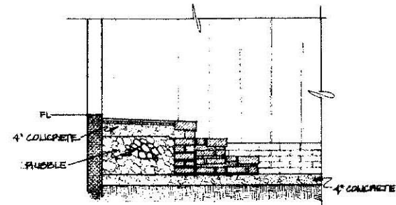
STEPS DETAIL SCALE: 1/2" = 1'-0"
