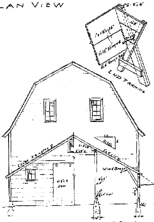
REAR END SECTION & ELEV.
