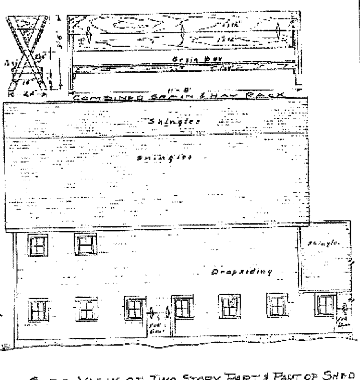
SIDE VIEW OF TWO STORY PART & PART OF SHED
