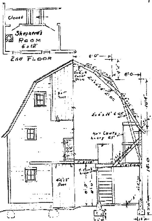
FRONT END SECTION
