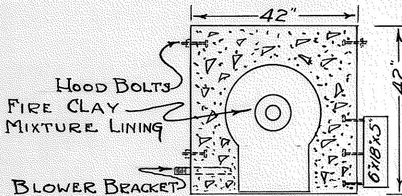
PLAN VIEW
