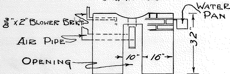
SCALE: \frac{1}{2} " = 1'-0" FRONT VIEW
