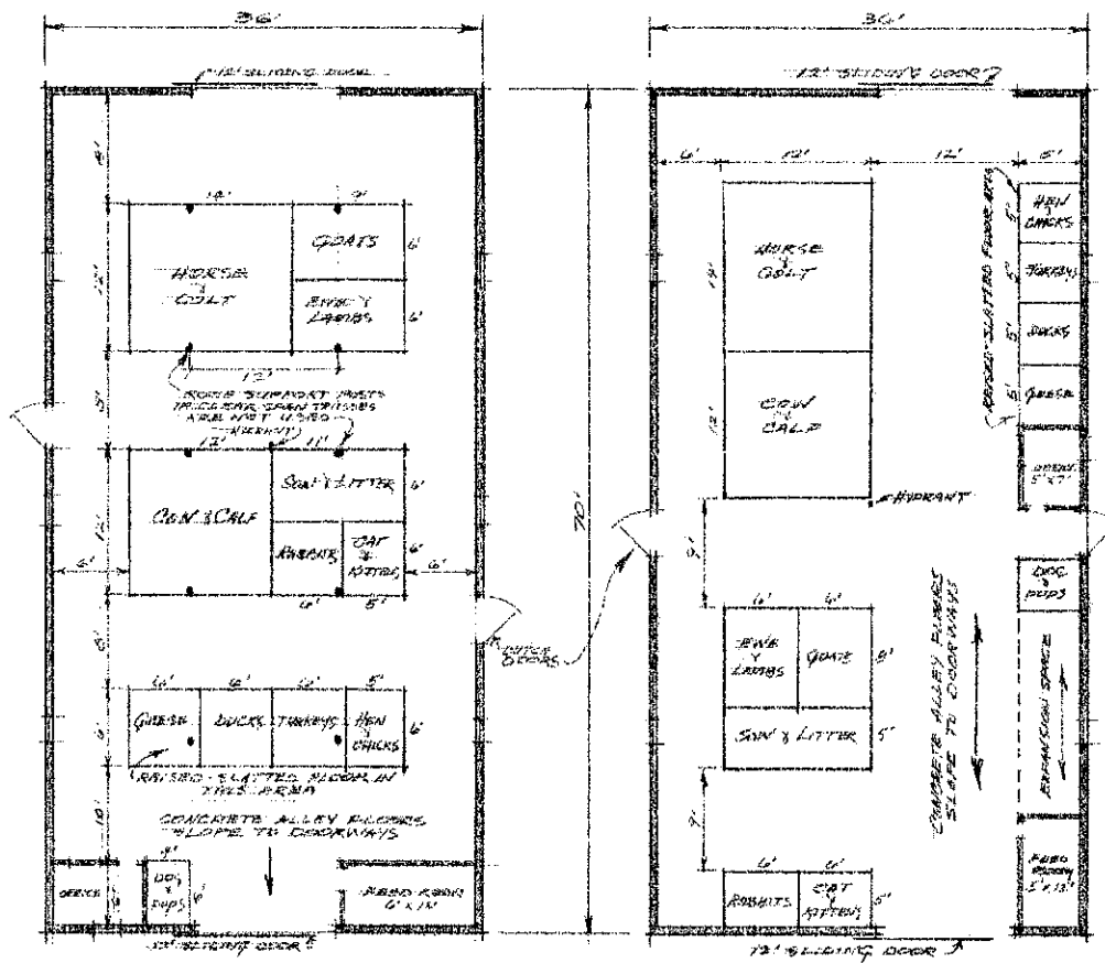
ALTERNATE FLOOR PLANS
