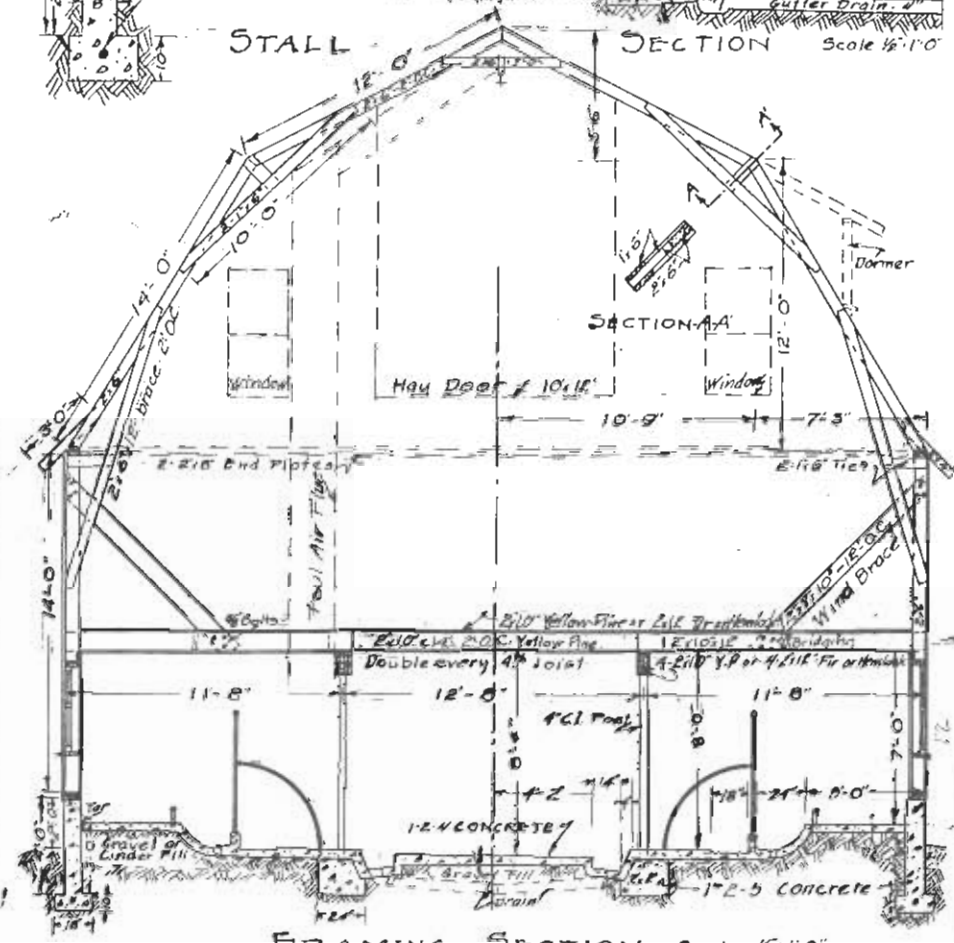
FRAMING SECTION Scale 1/4" = 1'-0"
