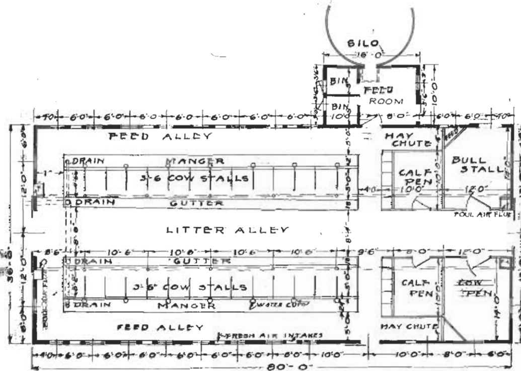
PLAN VIEW Scale 1/8" = 1'-0"
