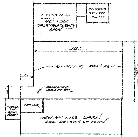
LAYOUT PLAN OF BARN'S
