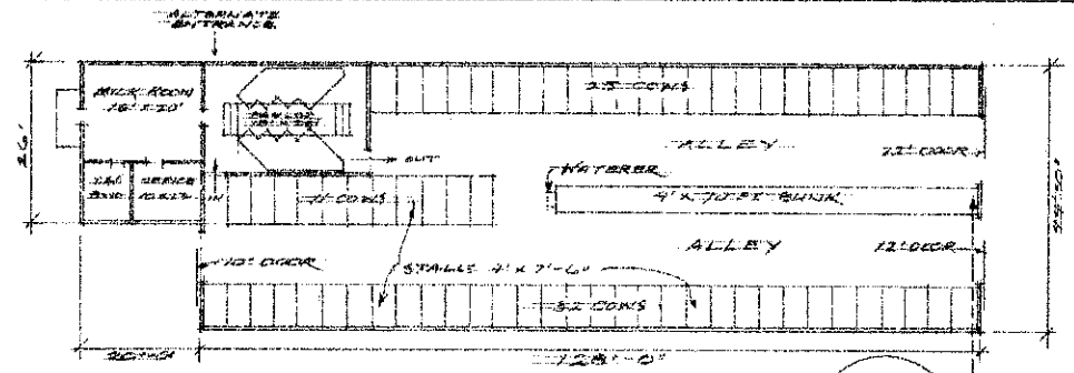
FLOOR PLAN DETAIL OF NEW 44' x 128' BARN
