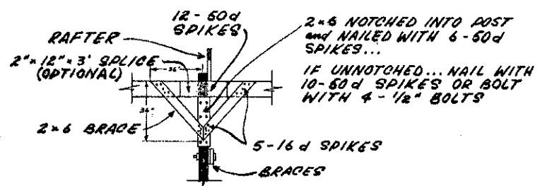
DETAIL OF BRACES AT PURLIN
