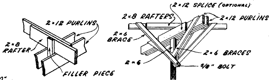
RAFTER TIE DETAIL
