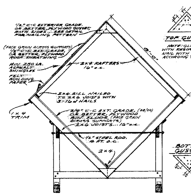
SECTION VIEW THRU BIN
