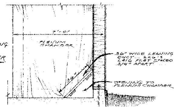
CROSS-SECTION A-A' SCALE: 1/2" = 1'-0"
