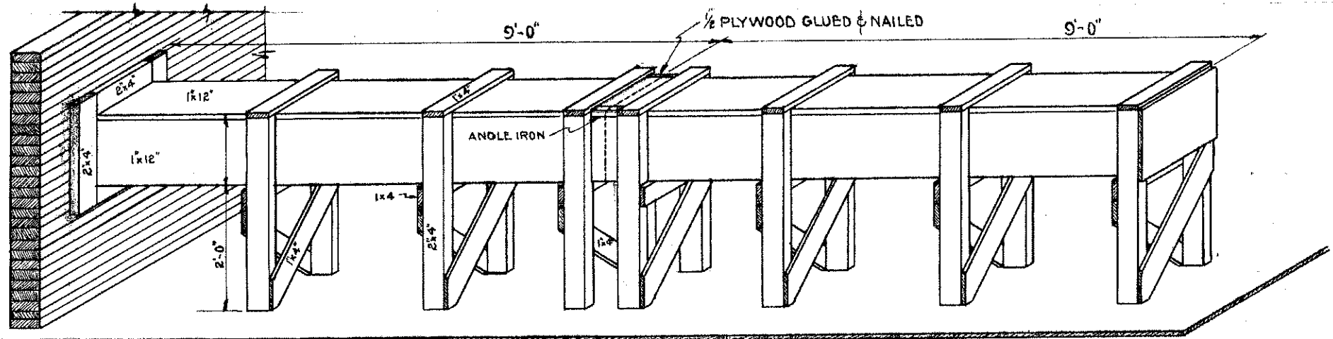
LATERAL DUCT ASSEMBLY DETAIL
