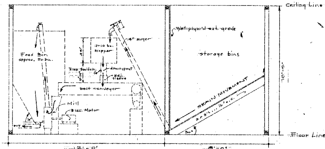
CROSS SECTION VIEW SCALE: 1/4" = 1'-0"
