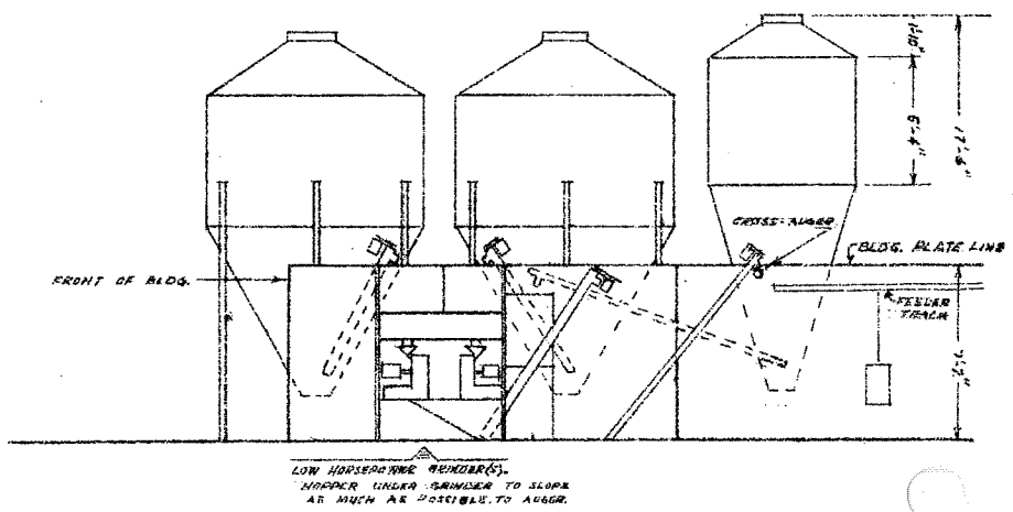
SIDE VIEW SCALE: 1/4"=1'-0"
