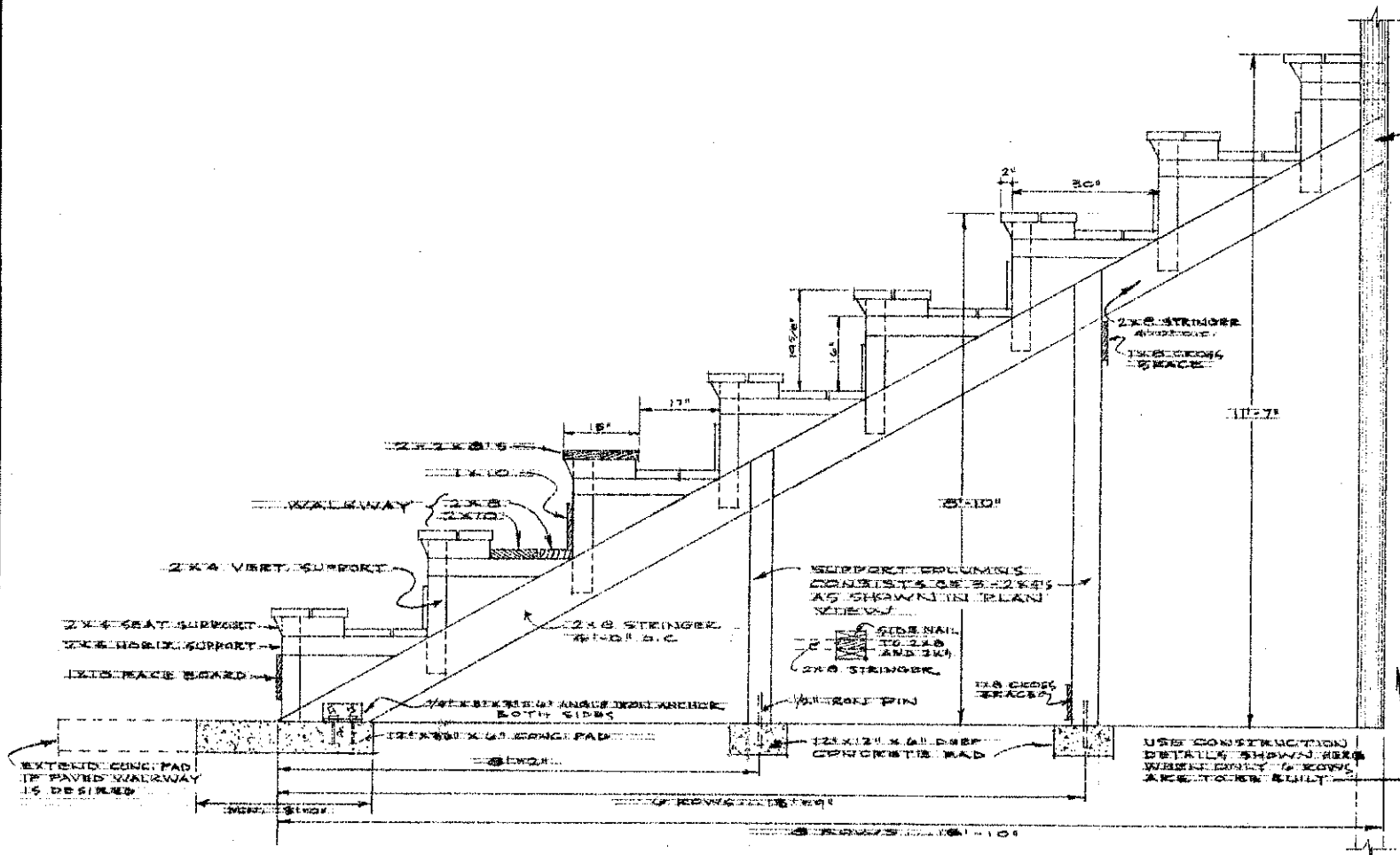
SIDE VIEW OF PERMANENT BLEACHERS SCALE: 3/4" = 1'-0"
