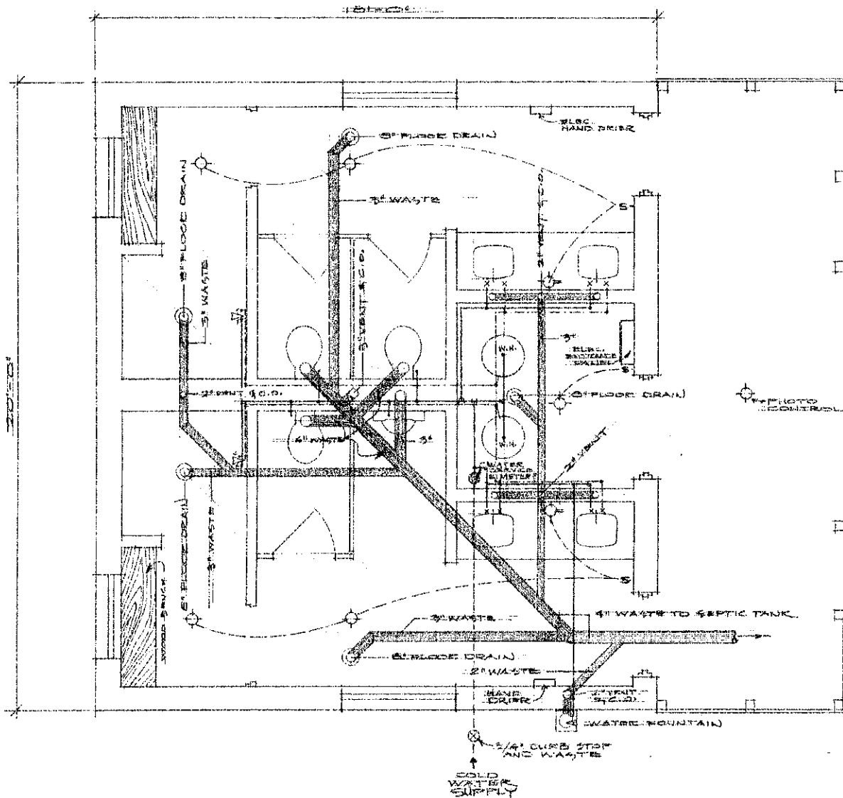
SEWER, WATER, AND ELECTRICAL PLAN SCALE: 1/2" = 1'-0"
