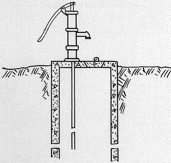
A DUG WELL PROPERLY PROTECTED
