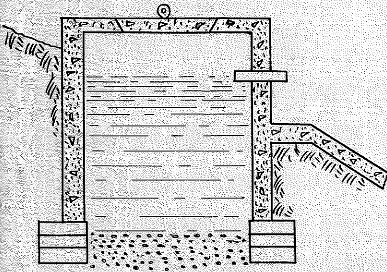
A SPRING PROPERLY PROTECTED
