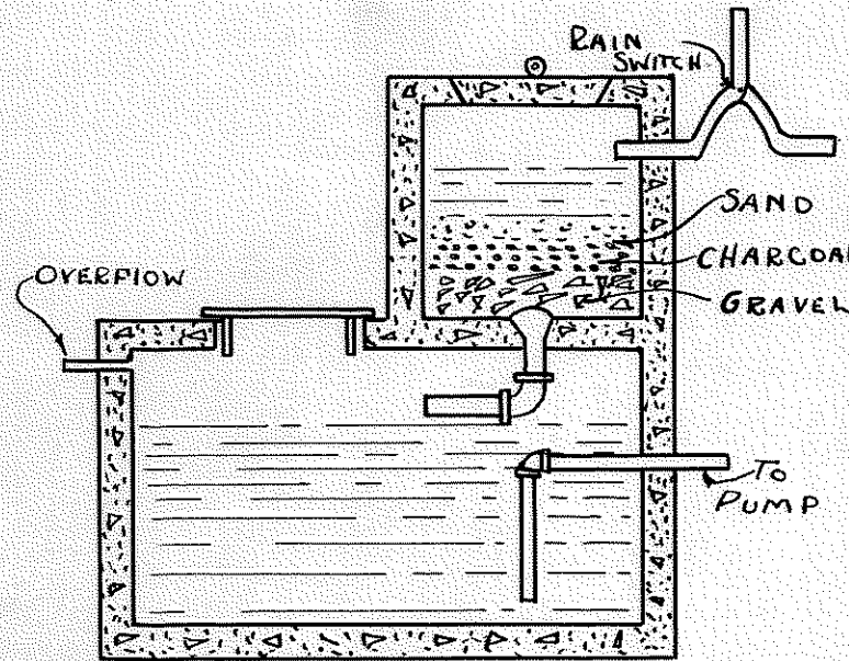
A CISTERN AND FILTER
