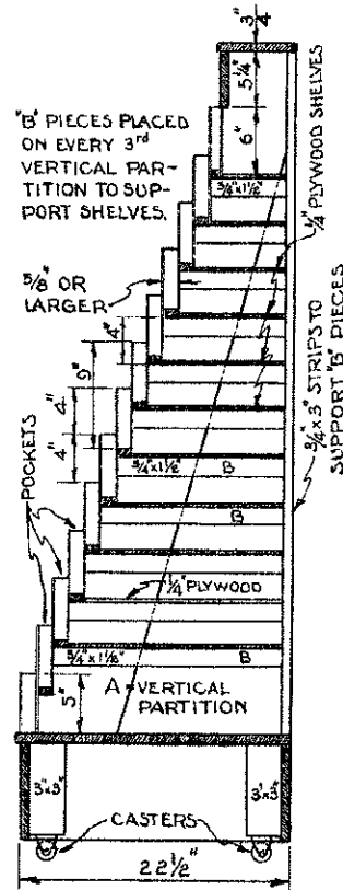
END VIEW-SECTION
