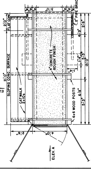
PLAN
