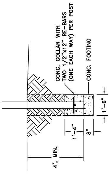
POST FOUNDATION DETAIL SCALE: 1/4"=1'-0"
