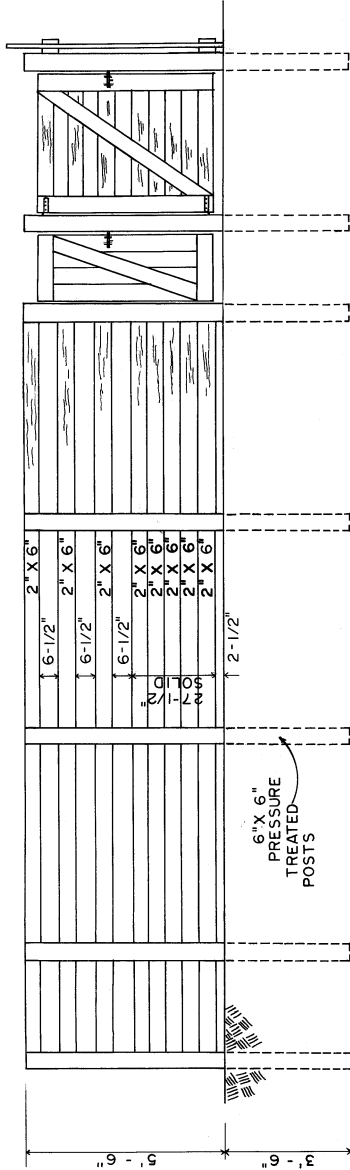
SIDE VIEW
