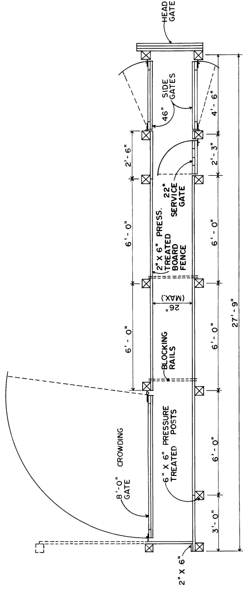
PLAN
