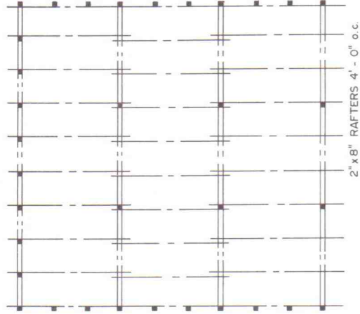
RAFTER LAYOUT
